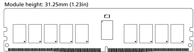
Figure 2: 288-Pin RDIMM (MO-309, R/C-C1)
