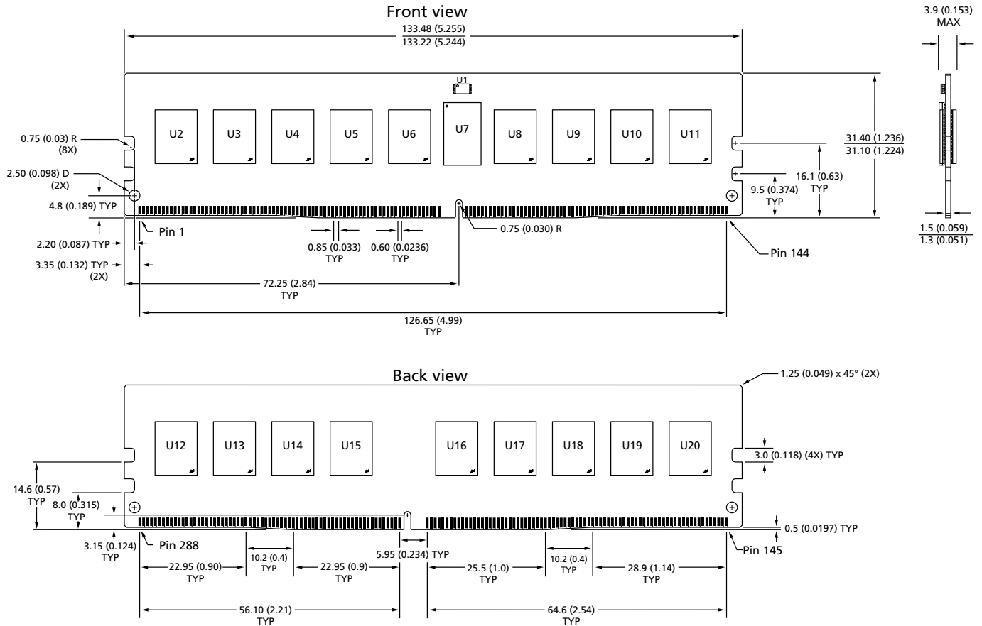
Figure 4: 288-Pin DDR4 RDIMM (R/C-C)
