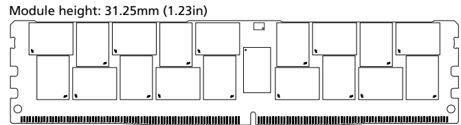
Figure 1: 288-Pin LRDIMM (MO-309, R/C-E1)
