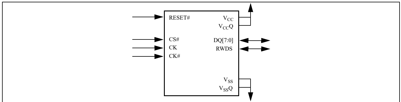
Figure 5 HYPERBUS™ interface [1]
