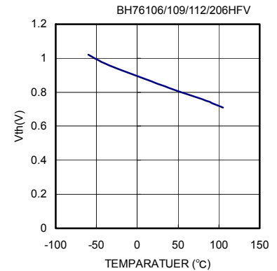
Fig.28 Temperature-V th
