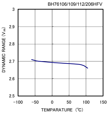
Fig.20 Dynamic Range Characteristic (Temperature Characteristic)
