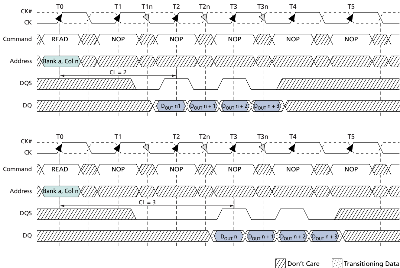
Figure 31: READ Burst
