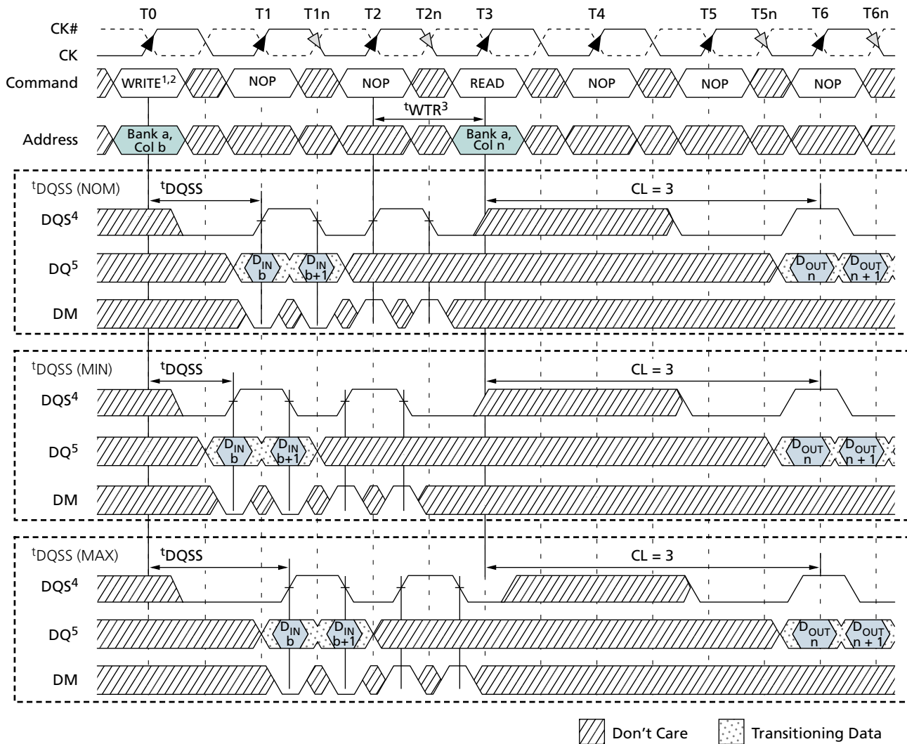
Figure 48: WRITE-to-READ – Interrupting
