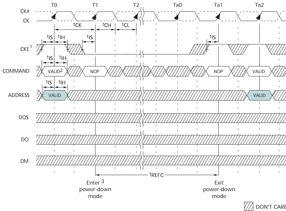
Figure 53: Power-Down Mode
