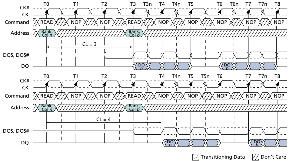
Figure 47: Nonconsecutive READ Bursts
