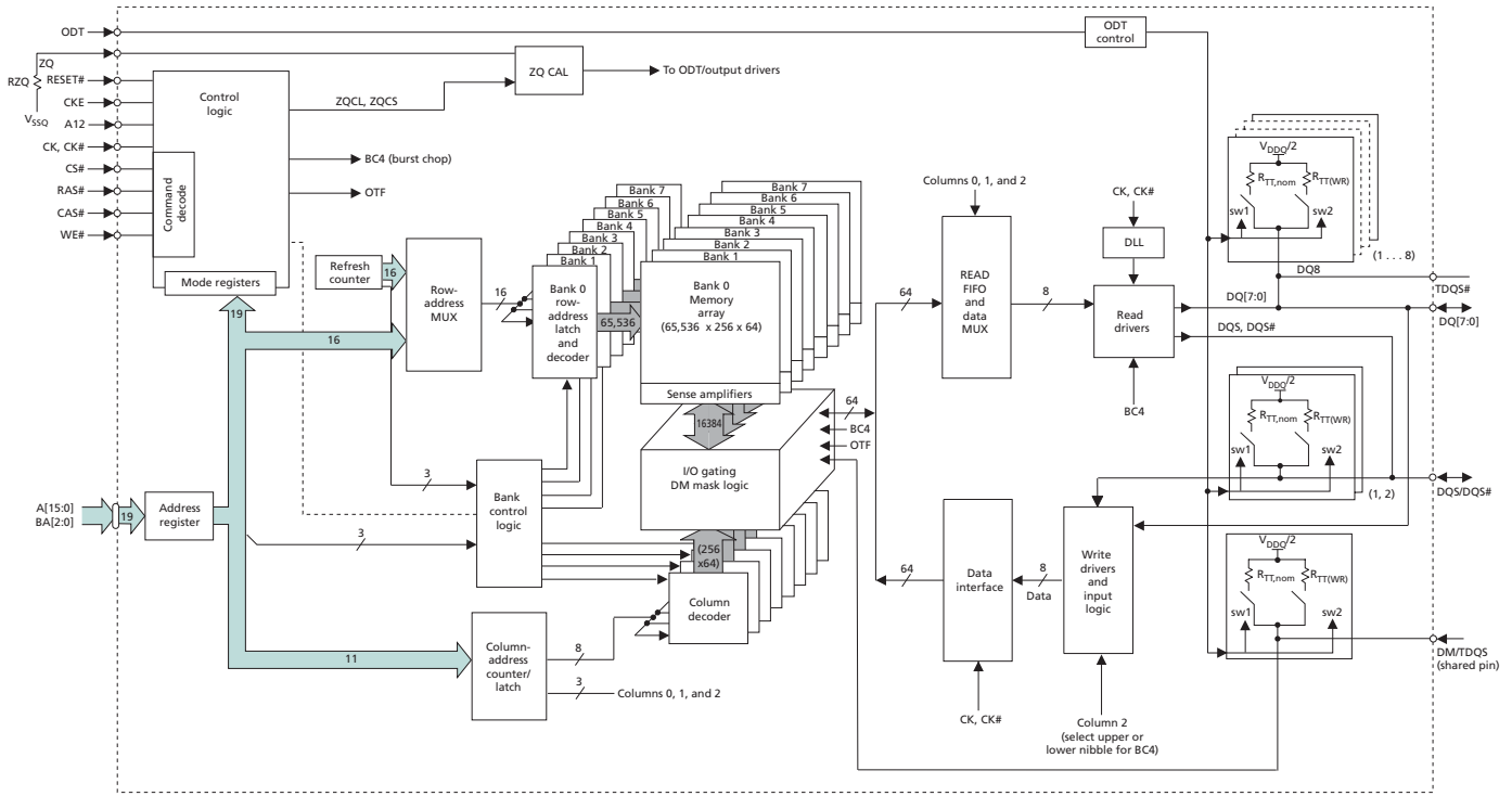
Figure 4: 1 Gig x 8 Functional Block Diagram
