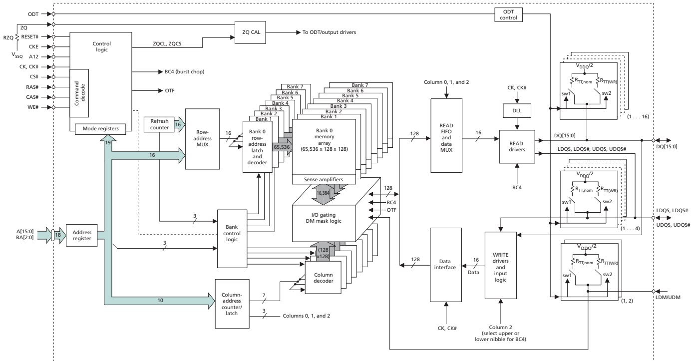
Figure 5: 512 Meg x 16 Functional Block Diagram
