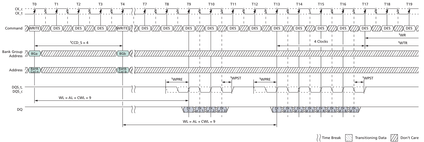
Figure 182: WRITE (BC4) OTF to WRITE (BL8) with 1^{\text{t}}\text{CK} Preamble in Different Bank Group
