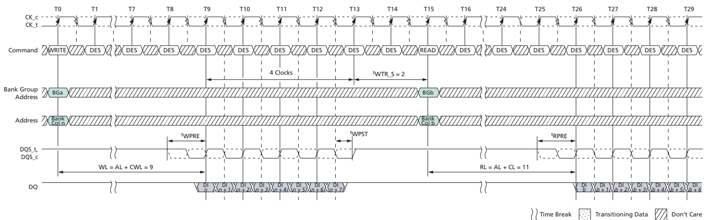
Figure 183: WRITE (BL8) to READ (BL8) with 1^{\text{t}}\text{CK} Preamble in Different Bank Group
