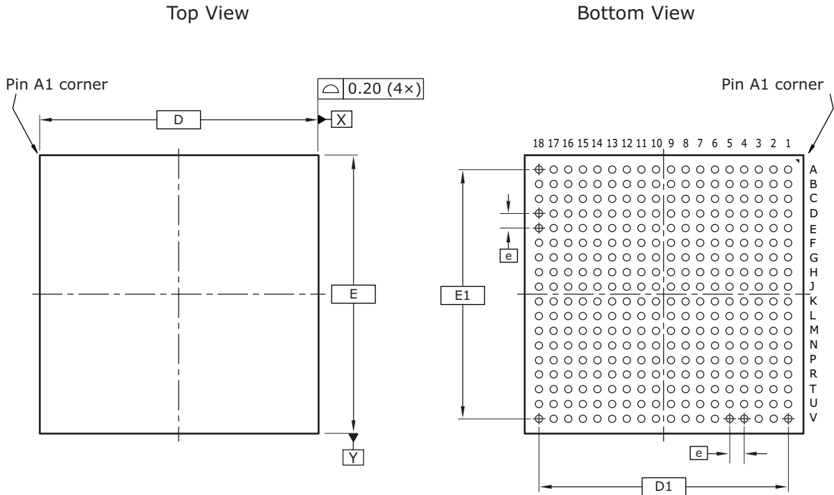
Figure 152 • Package Drawing
