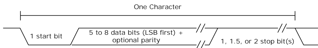
Figure 121 • UART Timing
