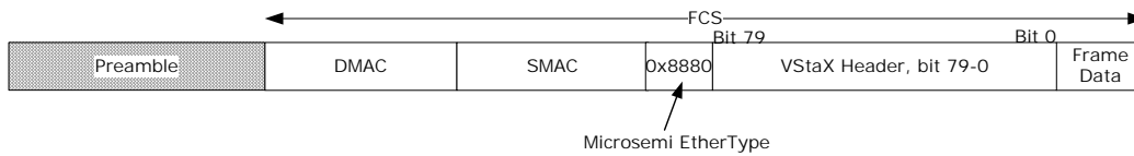
Figure 6 • Frame With VStaX Header
