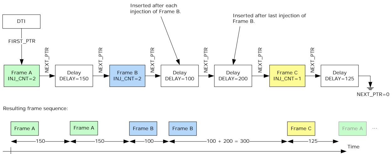
Figure 71 • DTI Frame/Delay Sequence Example
