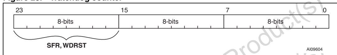
Figure 23. Watchdog counter
