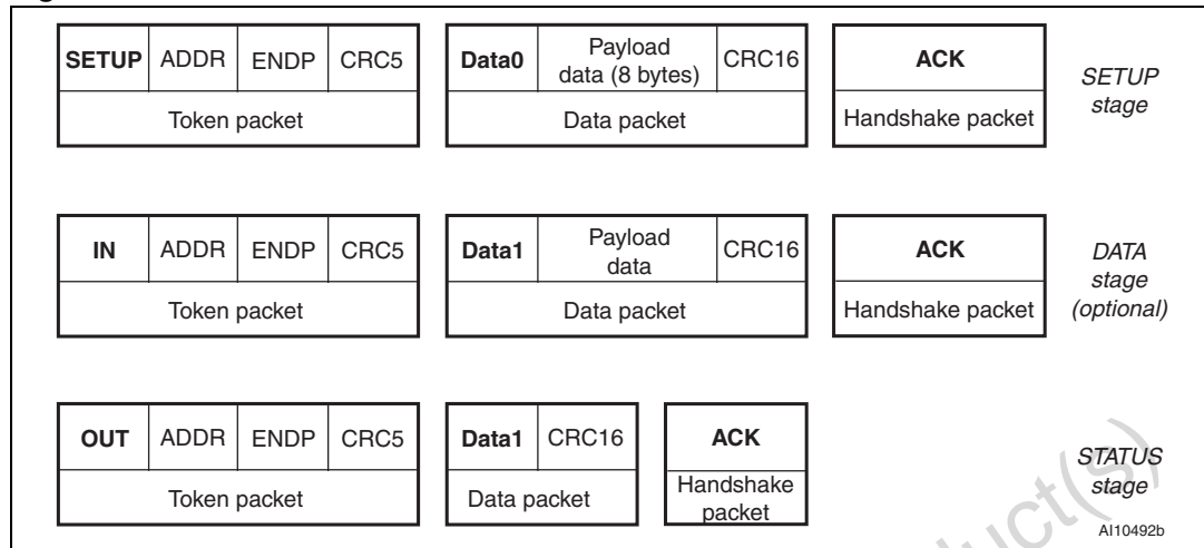
Figure 52. Control transfer
