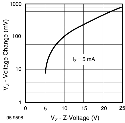
Fig. 3 - Typical Change of Working Voltage under Operating Conditions at T_{amb} = 25\text{ °C}
