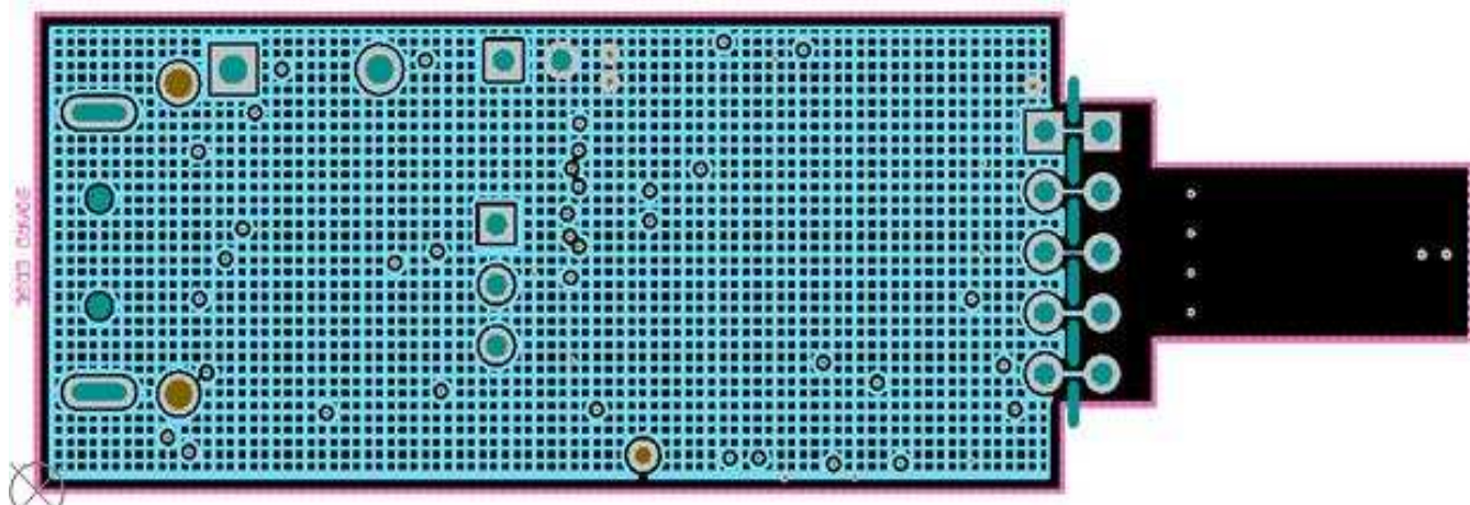
Figure 23. Power Layer Routing
