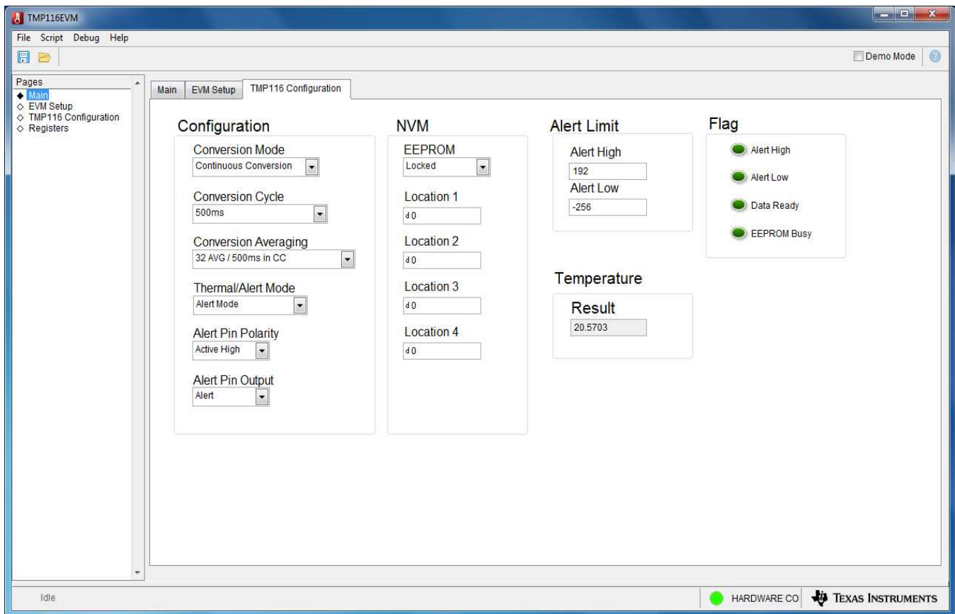
Figure 19. Configuration Tab
