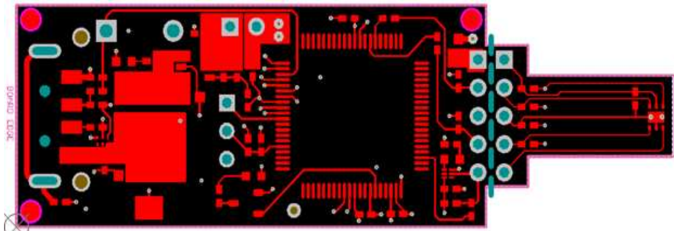
Figure 22. Top Layer Routing
