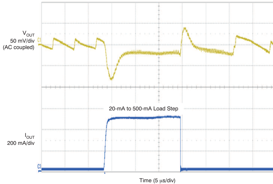
Figure 14. TLV62065 Transient Response, PFM Mode
