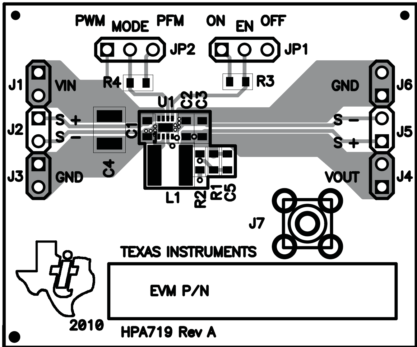
Figure 16. TLV62065EVM Component Placement, Top View
