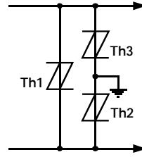
Figure 14. Multi-Point Protection
