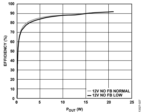
Figure 35. Efficiency vs. P_{OUT} , R_L = 4 \Omega , No FB and 220 pF, P_{VDD} = 12 V , Analog Gain = 12.6
