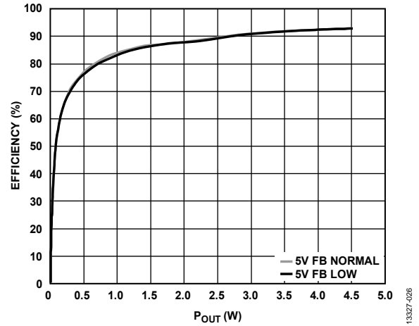
Figure 34. Efficiency vs. P_{OUT} , R_L = 4 \Omega , FB and 220 pF Capacitor, P_{VDD} = 5 V , Analog Gain = 8.4
