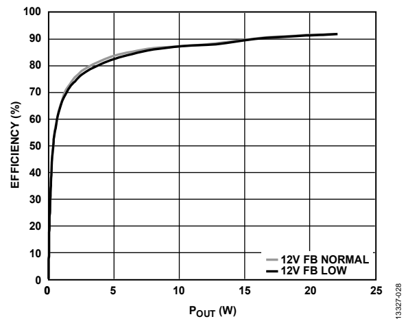
Figure 36. Efficiency vs. P_{OUT} , R_L = 4 \Omega , FB and 220 pF Capacitor, P_{VDD} = 12 V , Analog Gain = 12.6
