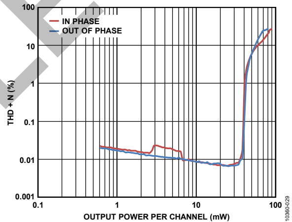
Figure 7. THD + N vs. Output Power, PVDD = 3.0 V, R_L = 16 \Omega
