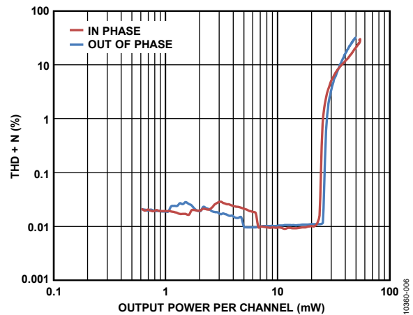
Figure 8. THD + N vs. Output Power, PVDD = 2.5 V, R_L = 16 \Omega
