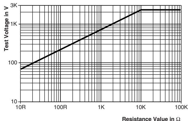
Pulse load rating in accordance with IEC 60 115-1, 4.27; 1.2 \mu s / 50 \mu s; 5 pulses at 12 s intervals; for permissible resistance change \pm (0.5 % R + 0.05 \Omega ) 1.2 / 50 Pulse
