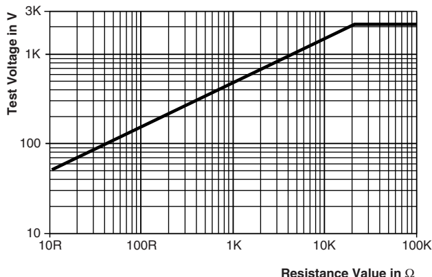
Pulse load rating in accordance with IEC 60115-1, 4.27; 10 \mu s / 700 \mu s; 10 pulses at 1 minute intervals; for permissible resistance change \pm (0.5 % R + 0.05 \Omega ) 10 / 700 Pulse
