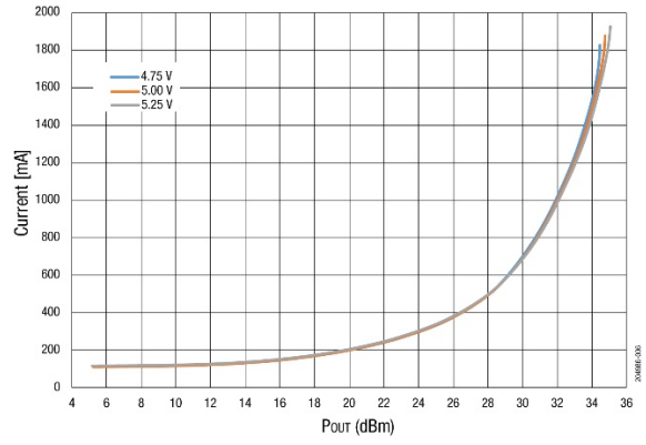
Figure 6. Iop vs Pout Across Vcc @ 3450 MHz, 25 °C
