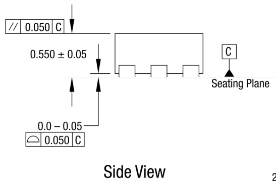
Figure 7. SKY65605-21 Package Dimensions
