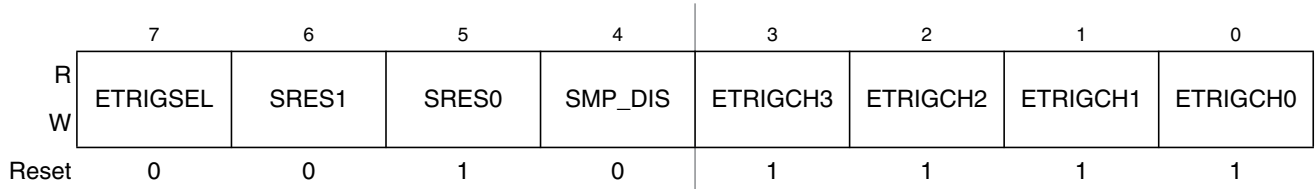
Figure 8-4. ATD Control Register 1 (ATDCTL1)
