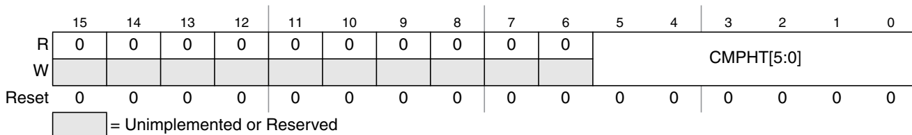
Figure 8-13. ATD Compare Higher Than Register (ATDCMPHT)
