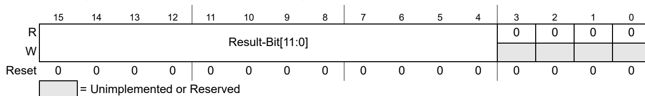
Figure 14-14. Left justified ATD conversion result register (ATDDRn)
