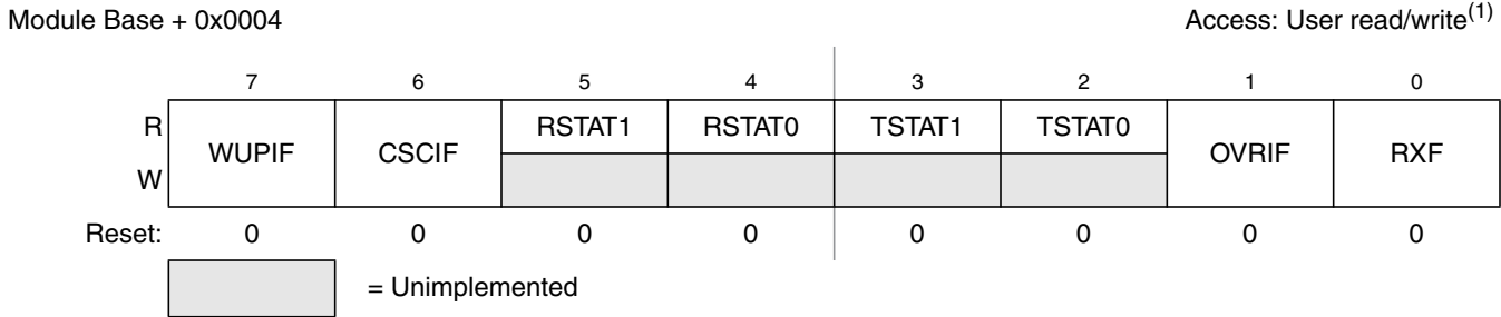
Figure 16-8. MSCAN Receiver Flag Register (CANRFLG)
