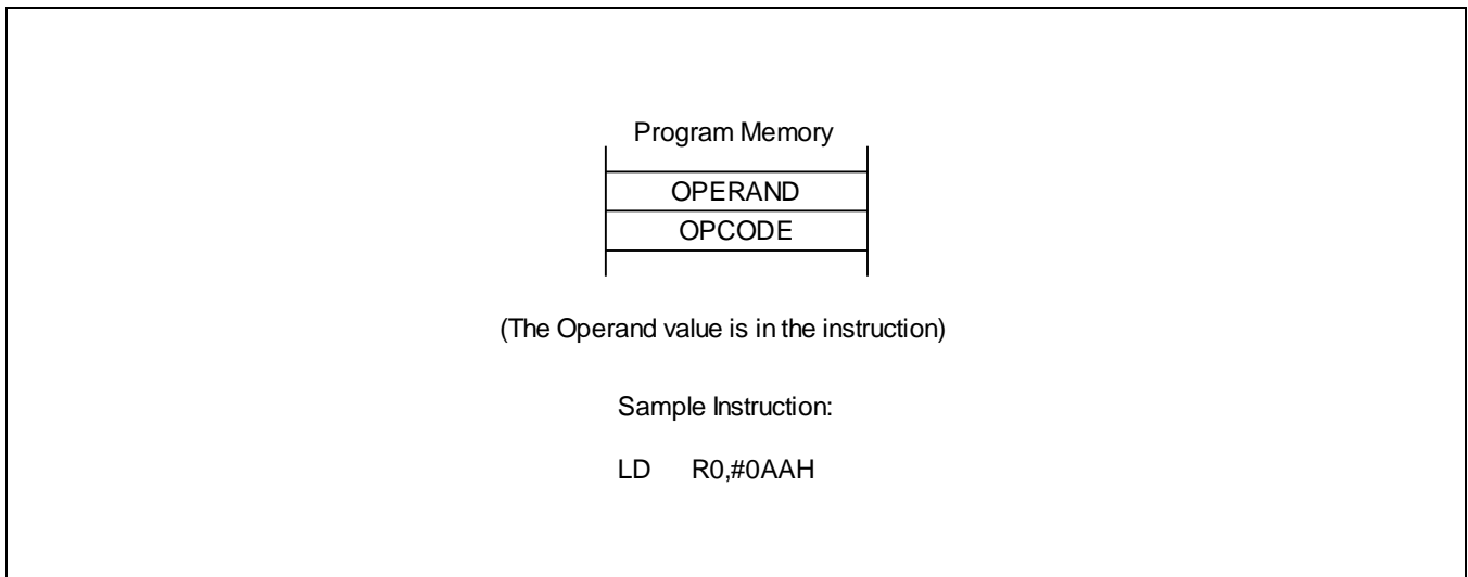
Figure 3-14 Immediate Addressing
