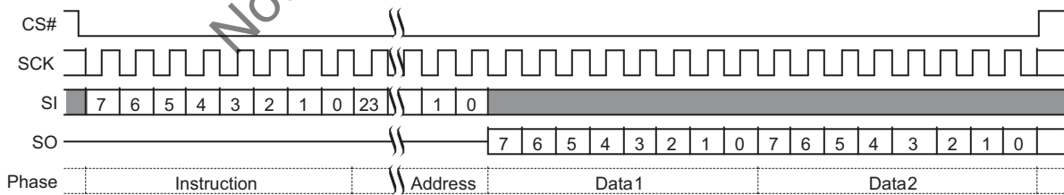
Figure 9. Single Bit Wide I/O Command without Latency
