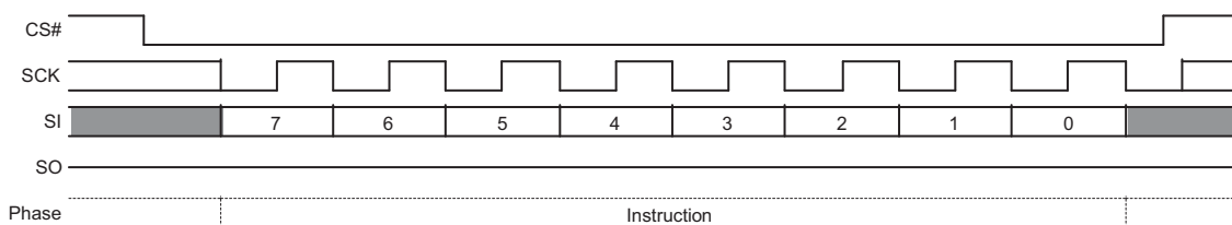
Figure 57. Release from Deep-Power-Down Command Sequence
