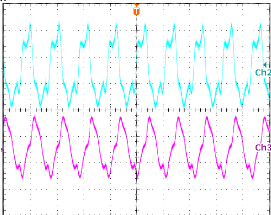
Output voltage ripple at nominal input voltage and max load current Top trace +15V, 10 mV/div, Bottom trace -15V, 20mV/div, 2us/div. Load cap: 10 \mu F, tantalum capacitor and 1 \mu F ceramic capacitor. Bandwidth: 20 MHz.
