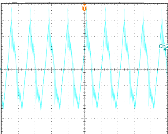
Output voltage ripple at nominal input voltage and max load current (5mV/div, 2us/div) Load cap: 10μF, tantalum capacitor and 1μF ceramic capacitor. Bandwidth: 20 MHz.
