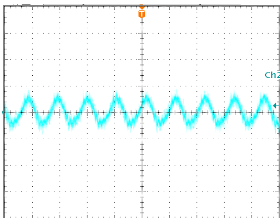
Output voltage ripple at nominal input voltage and max load current (4mV/div, 2us/div) Load cap: 10 \mu F, tantalum capacitor and 1 \mu F ceramic capacitor. Bandwidth: 20 MHz.
