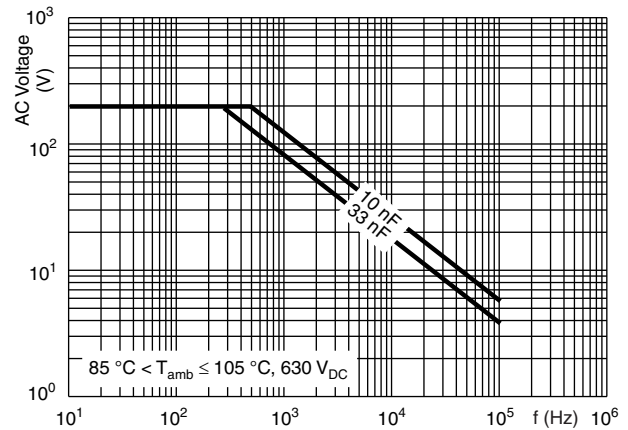
RMS voltage as a function of frequency
