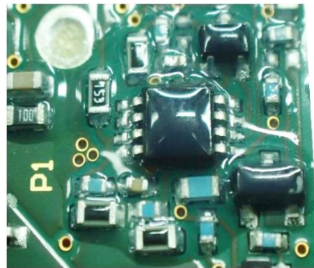
Fig 18: Actual picture of IC100 with conformal coating
