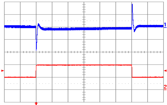
Fig. 10: Output voltage response to load current step-change (20 A – 30 A – 20 A) at V_{in} = 48\text{ V} . Top trace: output voltage (100 mV/div.). Bottom trace: load current (10 A/div.). Current slew rate: 5 A/ \mu\text{s} . C_o = 470\ \mu\text{F} POS + 1 \mu\text{F} ceramic. Time scale: 0.2 ms/div.
