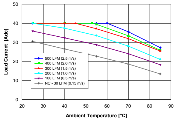
Fig. 2: Available load current vs. ambient air temperature and airflow rates for converter with G height pins mounted horizontally with air flowing from pin 1 to pin 3, MOSFET temperature \leq 120^\circ\text{C} , V_{in} = 48\text{ V}
