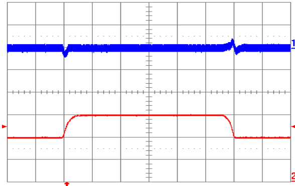
Fig. 9: Output voltage response to load current step-change (20 A – 20 A) at V_{in} = 48\text{ V} . Top trace: output voltage (100 mV/div.). Bottom trace: load current (10 A/div.). Current slew rate: 0.1 A/ \mu\text{s} C_o = 1\ \mu\text{F} ceramic. Time scale: 0.2 ms/div
