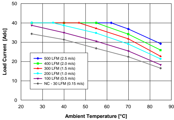
Fig. 1: Available load current vs. ambient air temperature and airflow rates for converter with G height pins mounted vertically with air flowing from pin 1 to pin 3, MOSFET temperature \leq 120^\circ\text{C} , V_{in} = 48\text{ V} Note: NC – Natural convection
