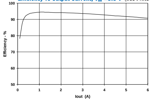
Efficiency vs Output Current, V_{in} = 3.3\text{ V} (See Note A)
