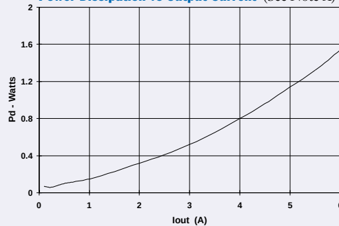
Power Dissipation vs Output Current (See Note A)
