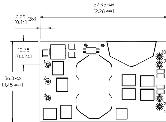
RECOMMENDED FOOTPRINT - TOP VIEW
