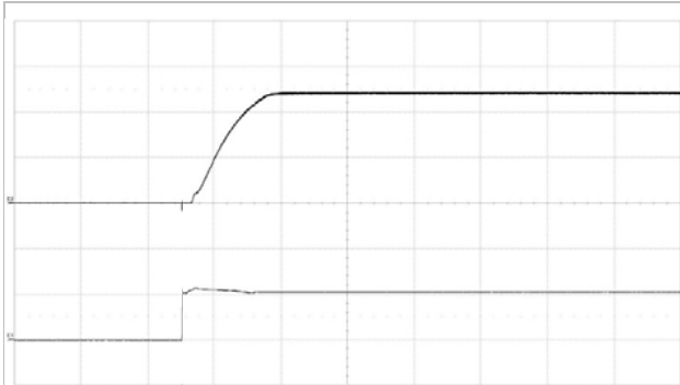
Start-up enabled by connecting V_I at: T_{P1} = +25^\circ\text{C} , V_I = 53\text{ V} , C_{out} = 2.2\text{ mF} I_O = 50\text{ A} resistive load.
