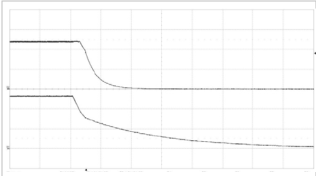
Shut-down enabled by disconnecting V_I at: T_{P1} = +25^\circ\text{C} , V_I = 53\text{ V} , C_{out} = 2.2\text{ mF} I_O = 50\text{ A} resistive load.
