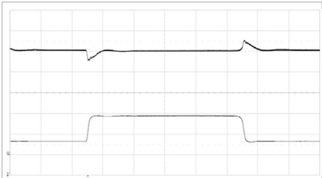
Output voltage response to load current step-change (12.5-37.5-12.5 A) at: T_{P1} = +25^\circ\text{C} , V_I = 53\text{ V} , C_{out} = 2.2\text{ mF}
