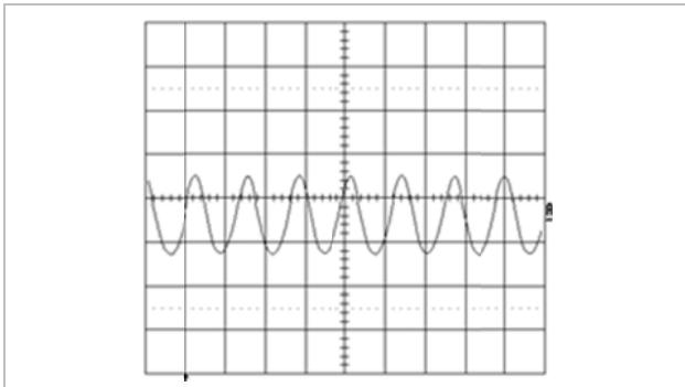
Output voltage ripple at: T_{P1} = +25^\circ\text{C} , V_I = 53\text{ V} , C_{out} = 2.2\text{ mF} I_O = 50\text{ A} resistive load.
