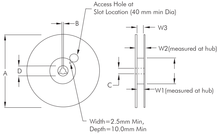
Figure 8-6 Reel Dimensions
