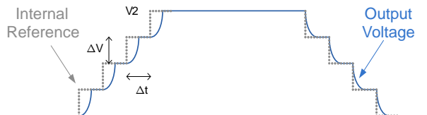
Figure 20. Dynamic Voltage Scaling Effect Timing
