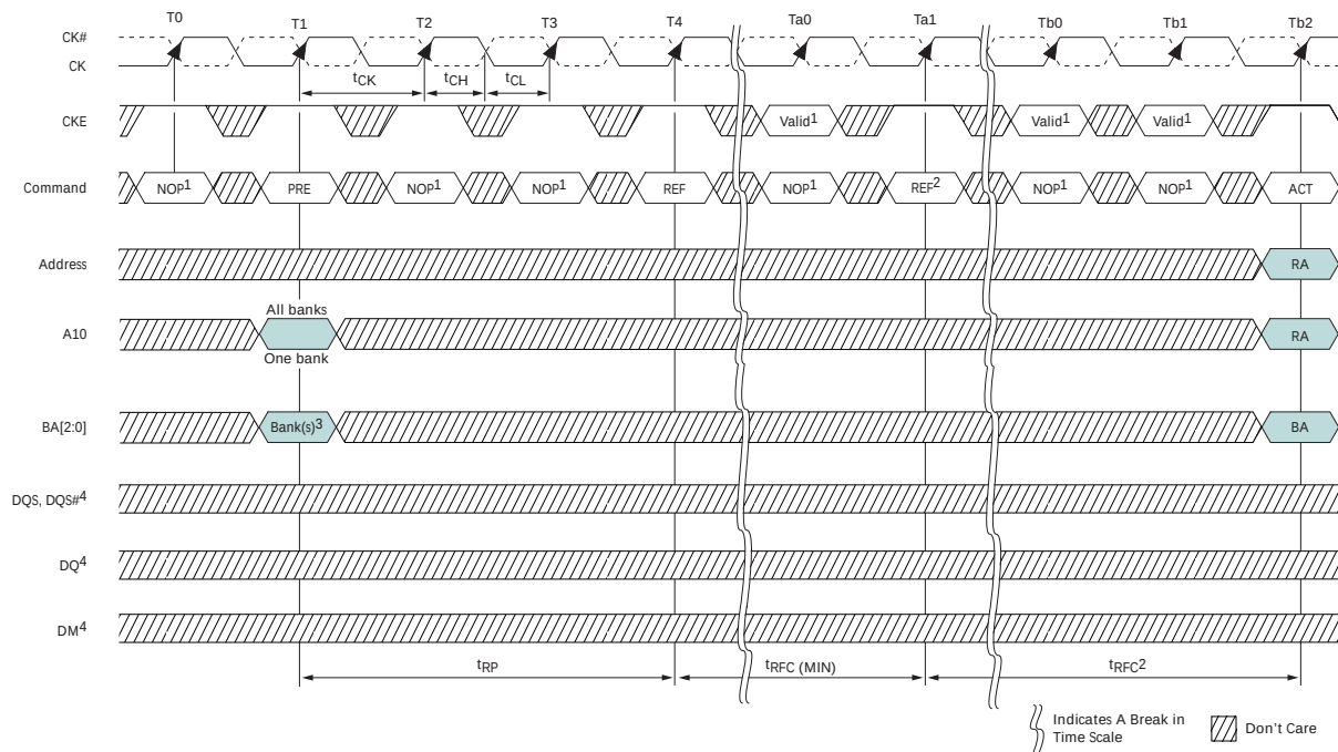
Figure 43: Refresh Mode
