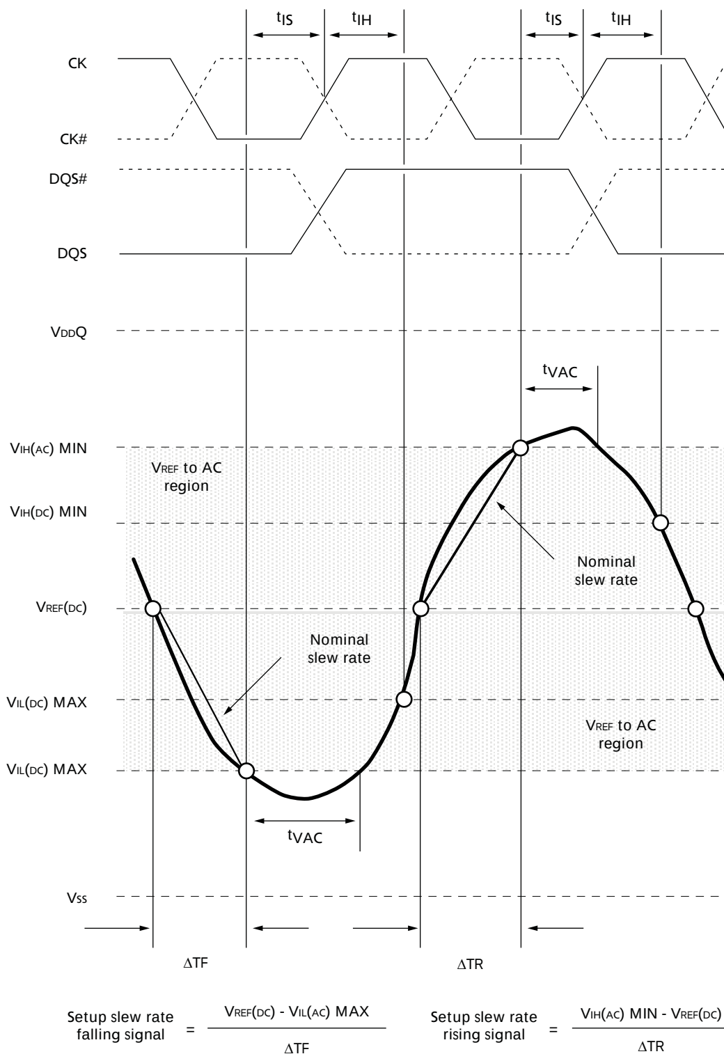
Figure 35: Nominal Slew Rate and t_{VAC} for t_{IS} (Command and Address – Clock)
