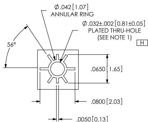
DETAIL "A" SCALE 8 : 1
