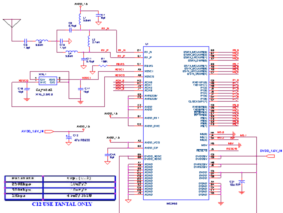
Figure 6. MG2450/MG2450A Application Circuit (I/O Power: 1.5V , MS[1]=1)
