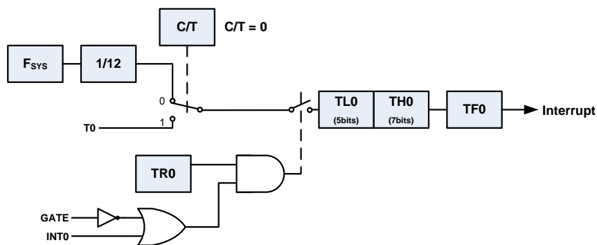
Figure 17. Timer0 Mode0
