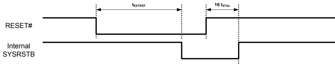
Figure 33. RESET# Timing
