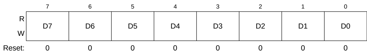
Figure 4-7. Linear Word Post Increment Register (LWP)
