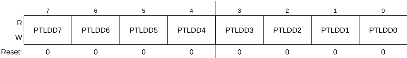
Figure 6-66. Port L Data Direction Register (PTLDD)
