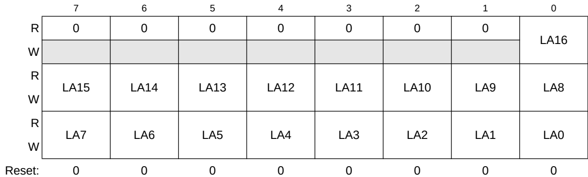
Figure 4-6. Linear Address Pointer Registers 2:0 (LAP2:LAP0)
