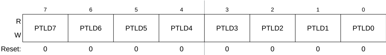
Figure 6-65. Port L Data Register (PTLD)
