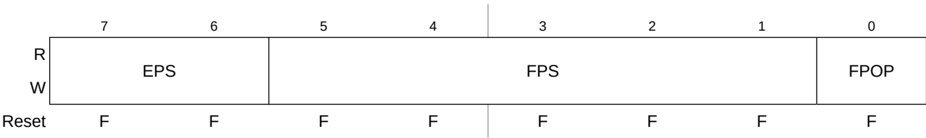
Figure 4-17. FLASH and EEPROM Protection Register (FPROT)
