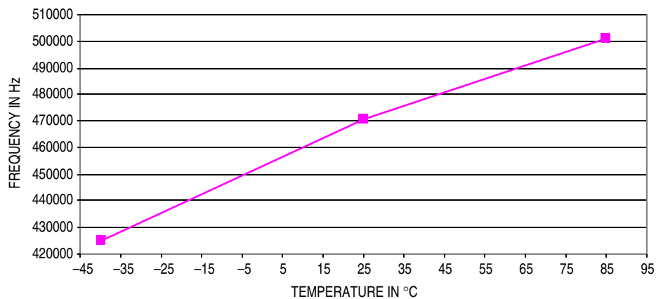
Figure 15-7. Typical 500 kHz External Low-Power Oscillator Frequency
