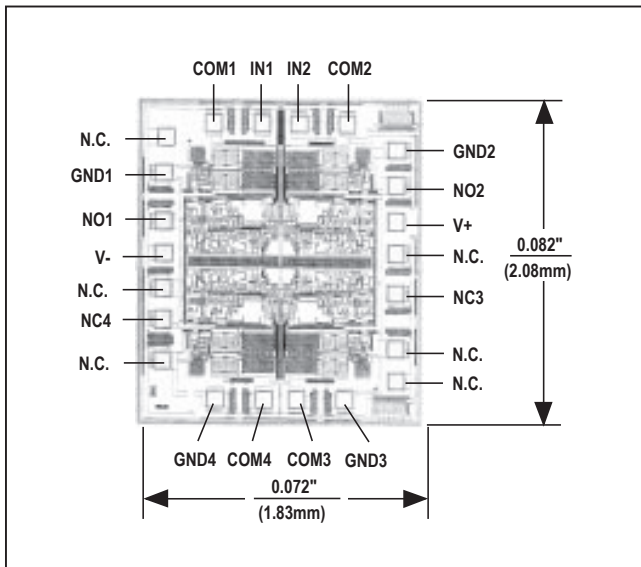
MAX4566
