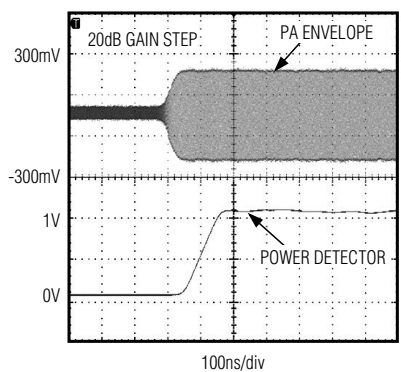
POWER-DETECTOR OUTPUT
