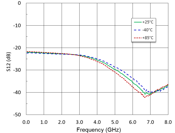
Reverse Isolation
