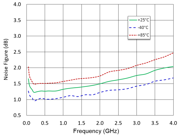
Noise Figure
