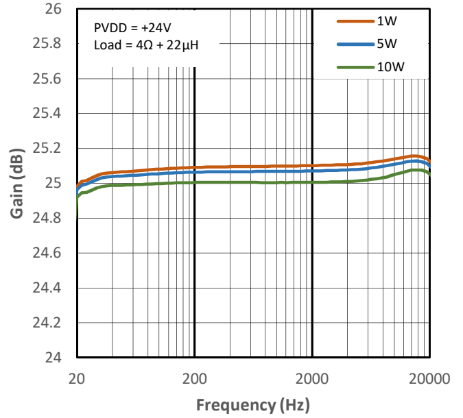
Figure 12-26 High Gain vs Frequency for PMP1
