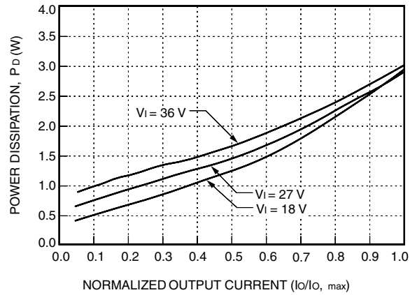
Figure 50. LC010A, B, C Typical Power Dissipation vs. Normalized Output Current at T_c = 25^\circ\text{C}
