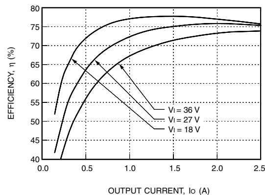
Figure 20. LC010F Typical Efficiency vs. Output Current at T_c = 25^\circ\text{C}
