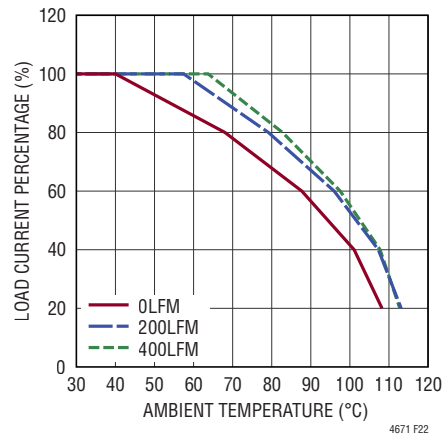
Figure 22. 5V IN Derating Curve, with Heat Sink CH0 and CH3 Paralleled to 1.8V/24A CH1 and CH2 Paralleled to 3.3V/10A
