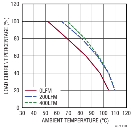
Figure 20. 12V IN Derating Curve, with Heat Sink CH0 and CH3 Paralleled to 1V/24A CH1 and CH2 Paralleled to 1.5V/10A
