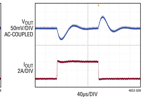
1V Transient Response, 24\text{V}_{\text{IN}}
