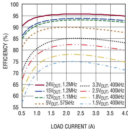
Efficiency vs Load Current at 36\text{V}_{\text{IN}} , Forced Continuous Mode
