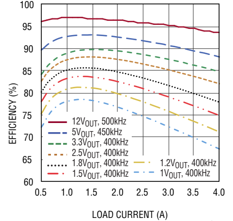
Efficiency vs Load Current at 15\text{V}_{\text{IN}} , Forced Continuous Mode
