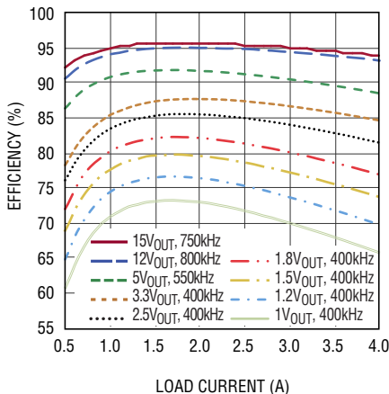
Efficiency vs Load Current at 24\text{V}_{\text{IN}} , Forced Continuous Mode
