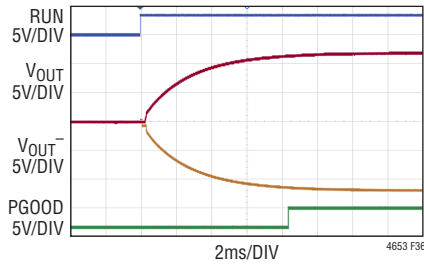
Figure 36. Concurrent ±12V Supply, Output Voltage Start-Up Waveforms, Figure 37 Circuit
