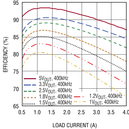
Efficiency vs Load Current at 12\text{V}_{\text{IN}} , Forced Continuous Mode
