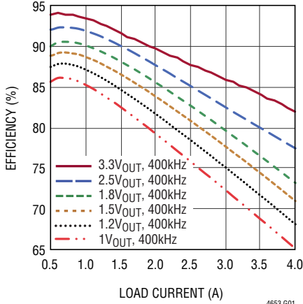
Efficiency vs Load Current at 5\text{V}_{\text{IN}} , Forced Continuous Mode
