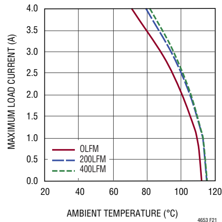
Figure 21. 48V to 5V OUT Derating Curve, No Heat Sink
