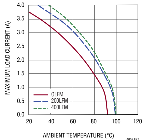
Figure 27. 48V to 24V OUT Derating Curve, No Heat Sink
