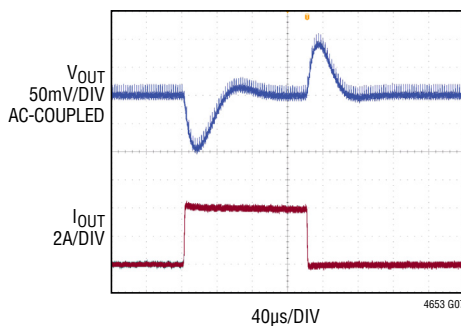
3.3V Transient Response, 48\text{V}_{\text{IN}}
