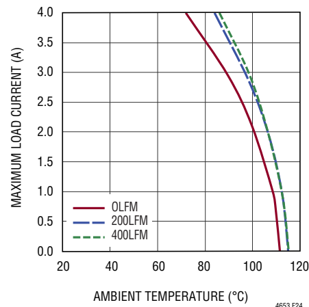
Figure 24. 48V to 5V OUT Derating Curve with BGA Heat Sink
