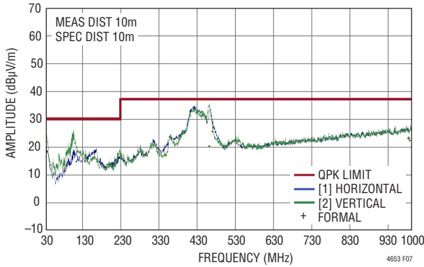
Figure 7. Radiated Emissions Scan of the LTM4653 Producing 24V OUT at 3.5A, from 48V IN , DC2327A Hardware, f SW = 1.2MHz, Measured in a 10m Chamber, Peak Detect Method
