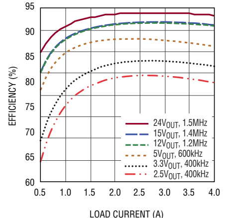
Efficiency vs Load Current at 48\text{V}_{\text{IN}} , Forced Continuous Mode
