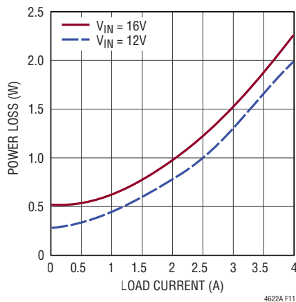
Figure 11. 8V Output Power Loss
