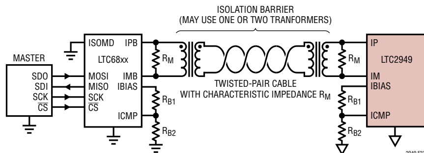
Figure 23. isoSPI Circuit
