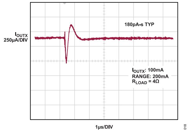
Figure 18. Mid-Scale Glitch
