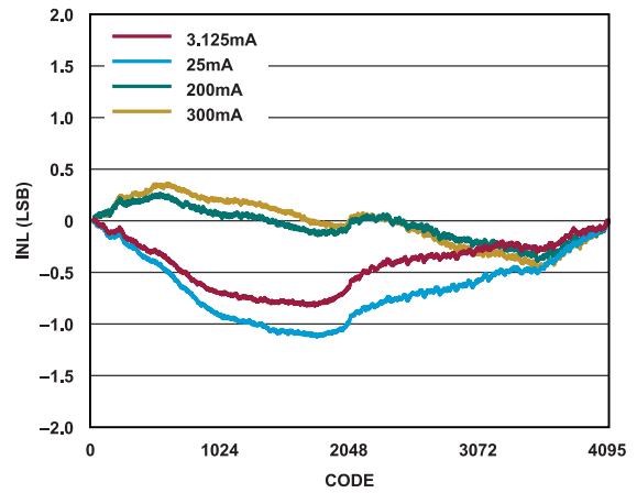
Figure 23. LTC2662-12 Integral Nonlinearity (INL)
