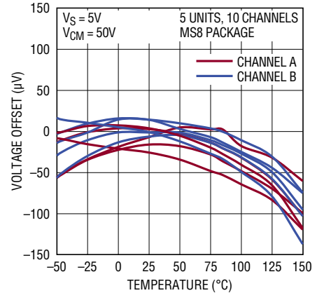
Over-The-Top Voltage Offset vs Temperature
