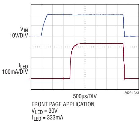
Turn ON and OFF Performance
