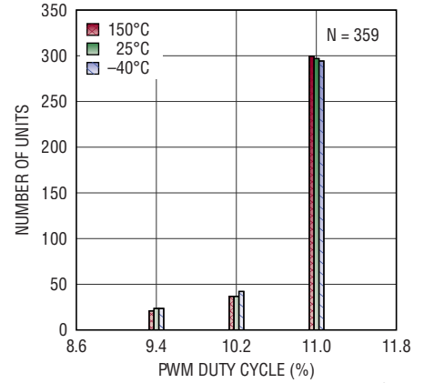
Internal PWM Duty Cycle (10%)
