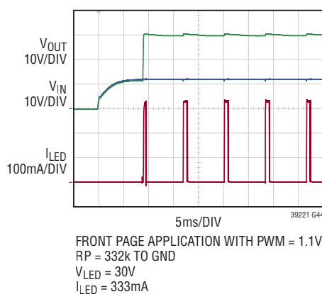
Start-Up with 10% Internal PWM
