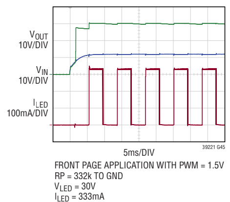
Start-Up with 50% Internal PWM
