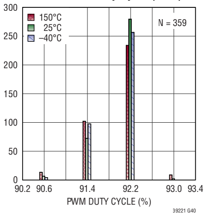
Internal PWM Duty Cycle (90%)
